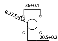
Panel drilling
