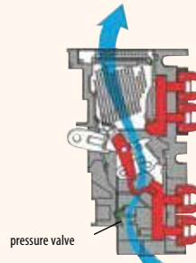
Efficient air convection through a pressure valve
