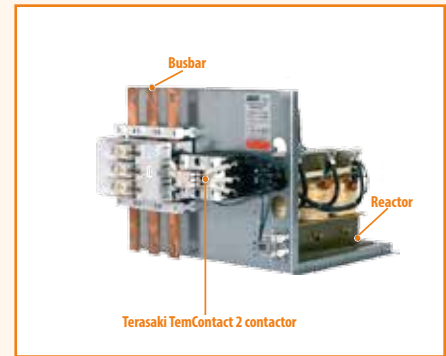
Modular Cassette Unit
